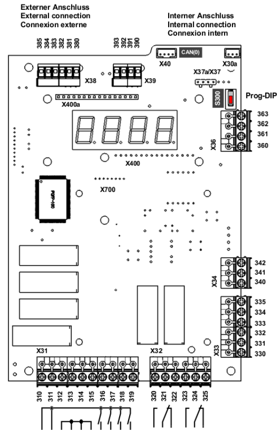
Abb./Fig. 4: Anschlüsse/Connections/Raccordements
